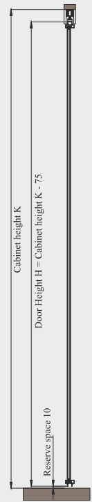
Al. Frame Door
