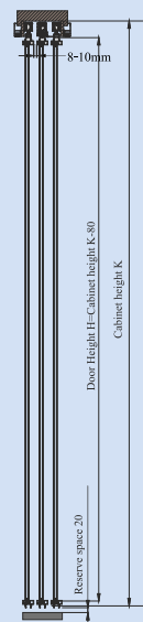
Al. Frame Door
